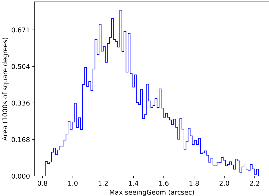
roll_pause_mjdp60_v3.4_10yrs Yr 1 r band: Max seeingGeom
