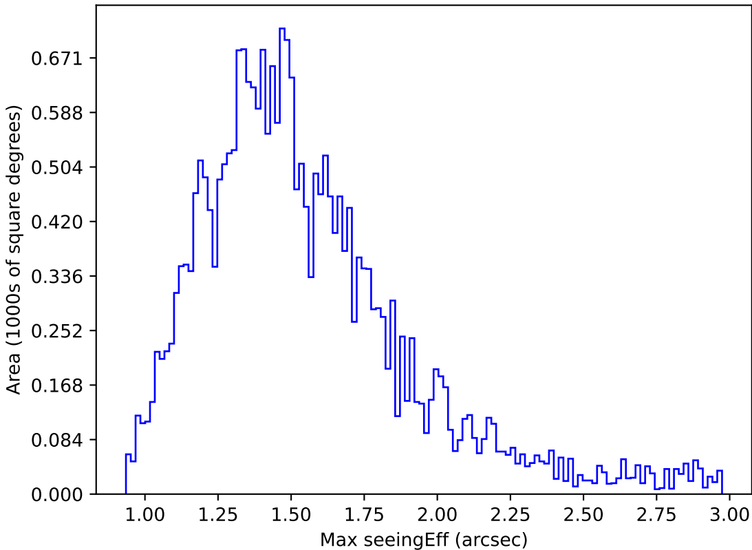
roll_pause_mjdp60_v3.4_10yrs Yr 1 z band: Max seeingEff
