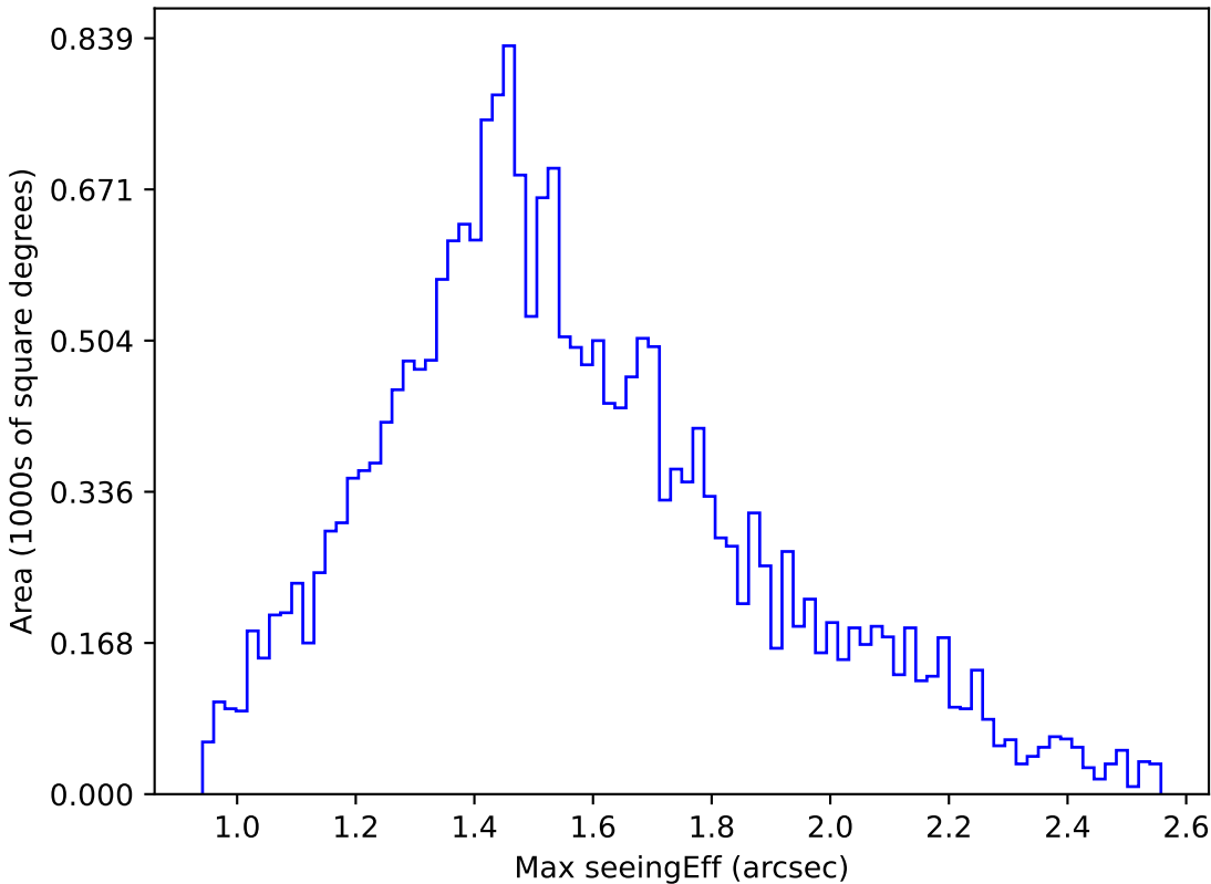
roll_pause_mjdp60_v3.4_10yrs Yr 1 u band: Max seeingEff
