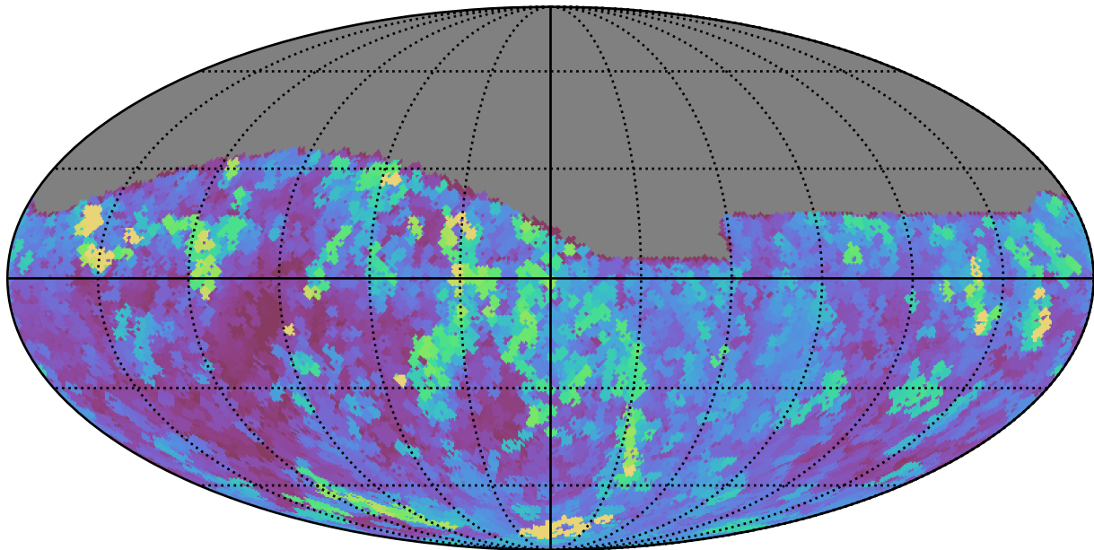
roll_pause_mjdp60_v3.4_10yrs Yr 1 all bands: Max seeingEff
