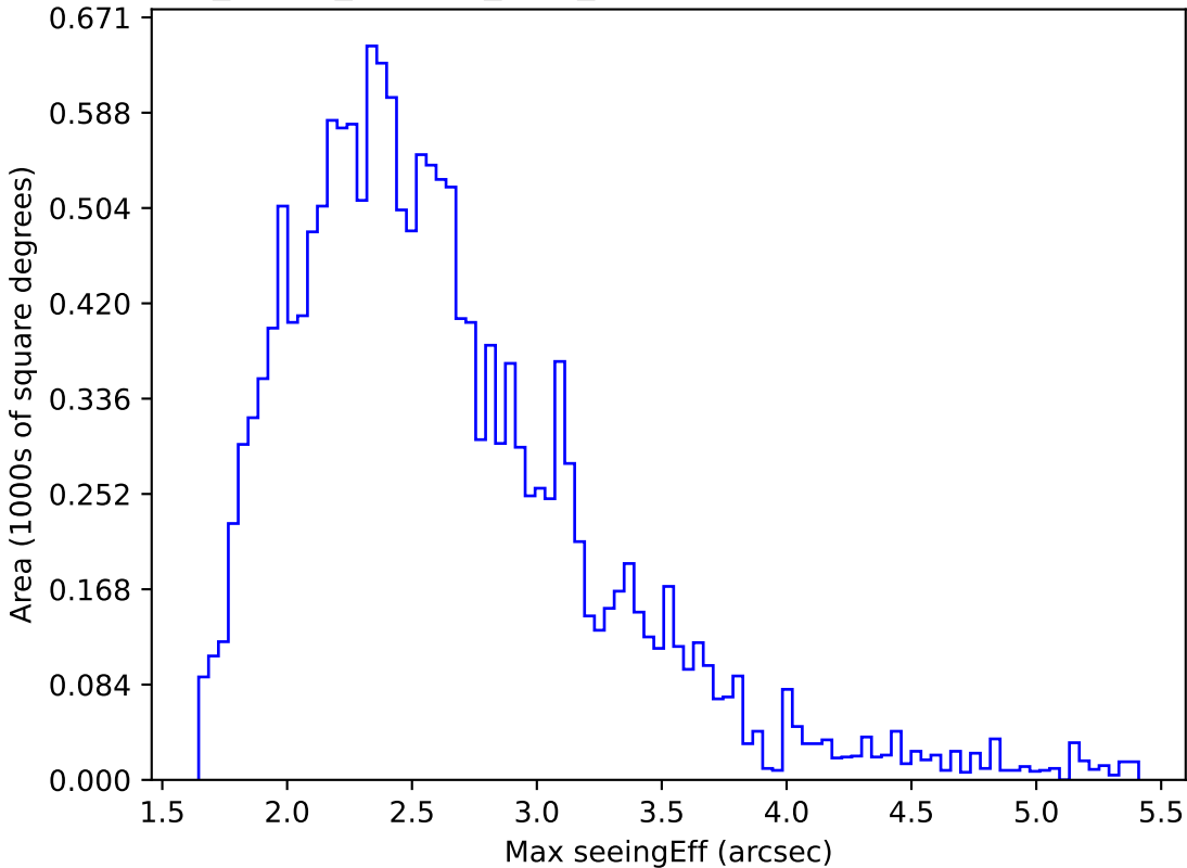
roll_pause_mjdp60_v3.4_10yrs WFD z band: Max seeingEff
