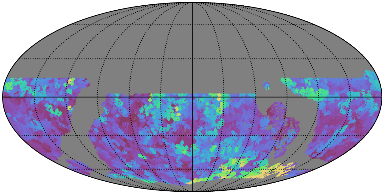
roll_pause_mjdp60_v3.4_10yrs WFD u band: Max seeingEff
