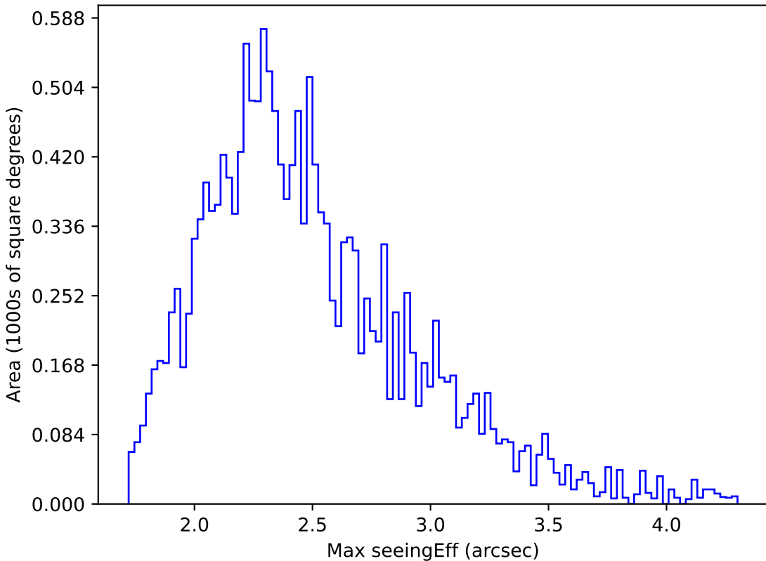
roll_pause_mjdp60_v3.4_10yrs WFD u band: Max seeingEff
