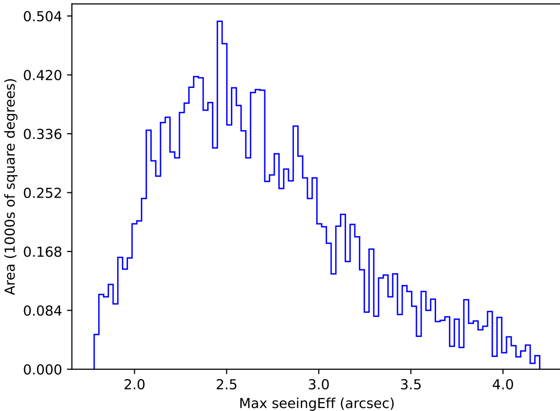
roll_pause_mjdp60_v3.4_10yrs WFD r band: Max seeingEff
