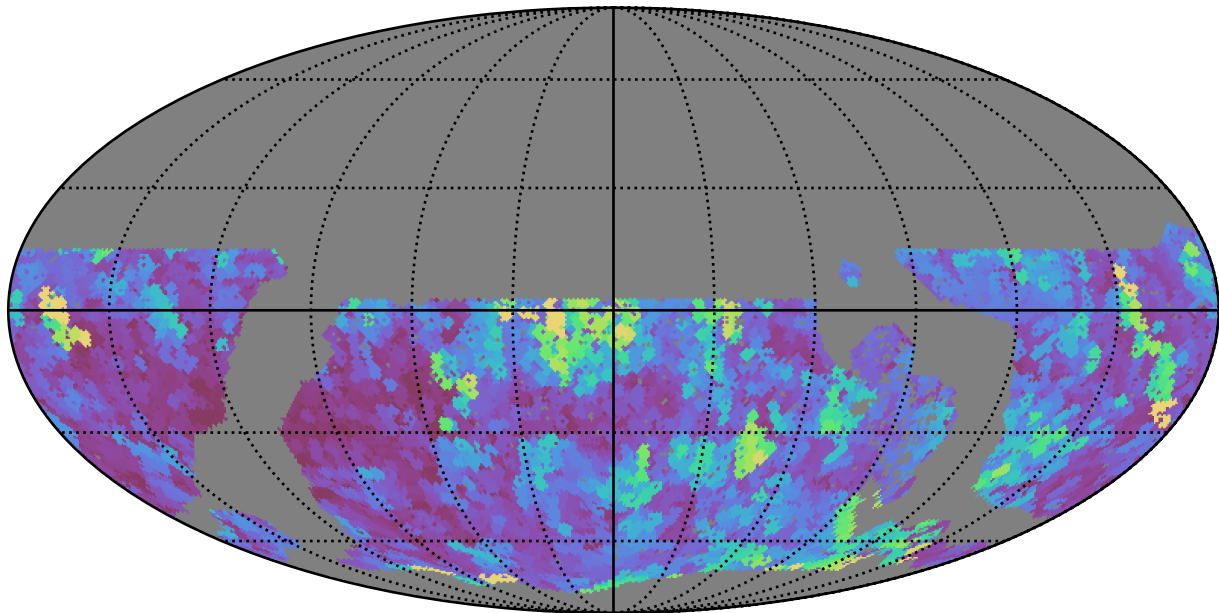
roll_pause_mjdp60_v3.4_10yrs WFD all bands: Max seeingEff
