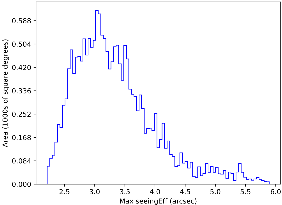
roll_pause_mjdp60_v3.4_10yrs WFD all bands: Max seeingEff
