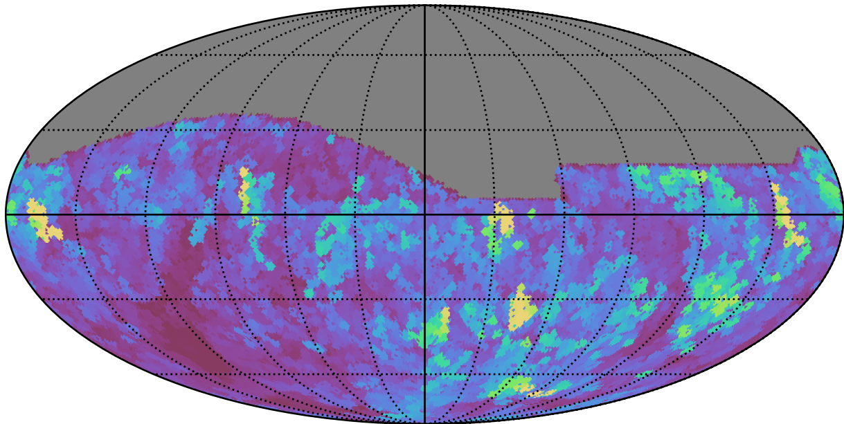
roll_pause_mjdp60_v3.4_10yrs All sky z band: Max seeingEff
