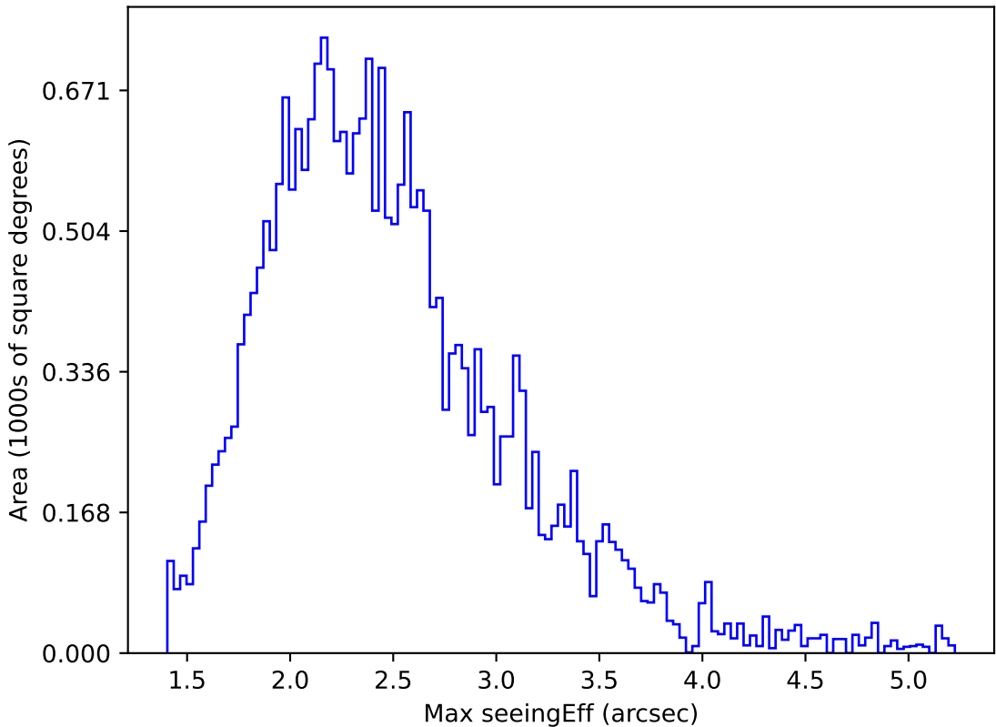
roll_pause_mjdp60_v3.4_10yrs All sky z band: Max seeingEff
