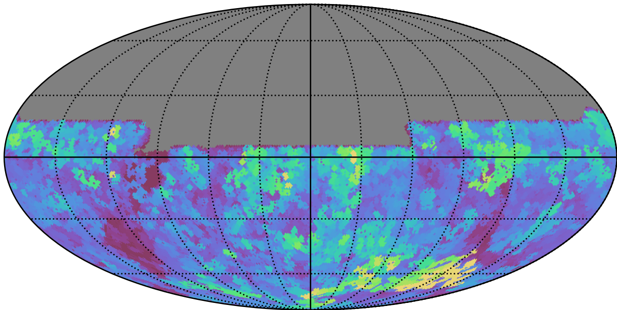
roll_pause_mjdp60_v3.4_10yrs All sky u band: Max seeingEff
