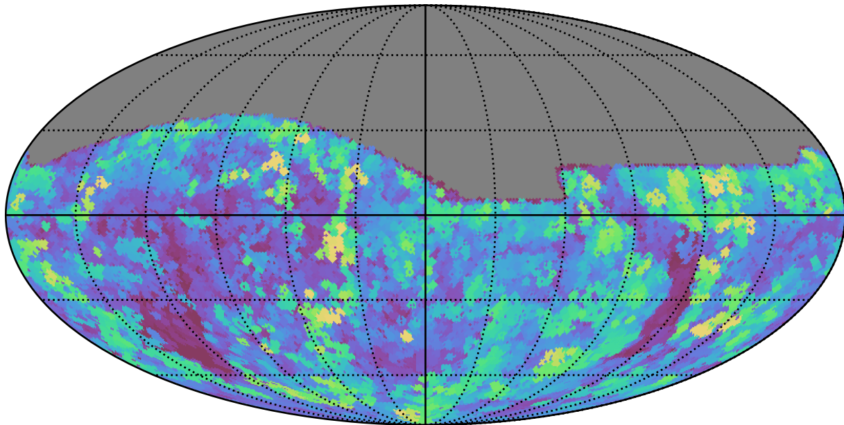
roll_pause_mjdp60_v3.4_10yrs All sky g band: Max seeingEff
