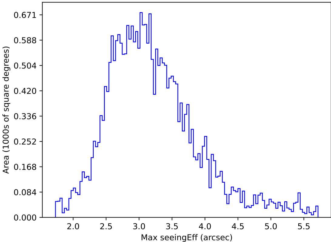
roll_pause_mjdp60_v3.4_10yrs All sky all bands: Max seeingEff
