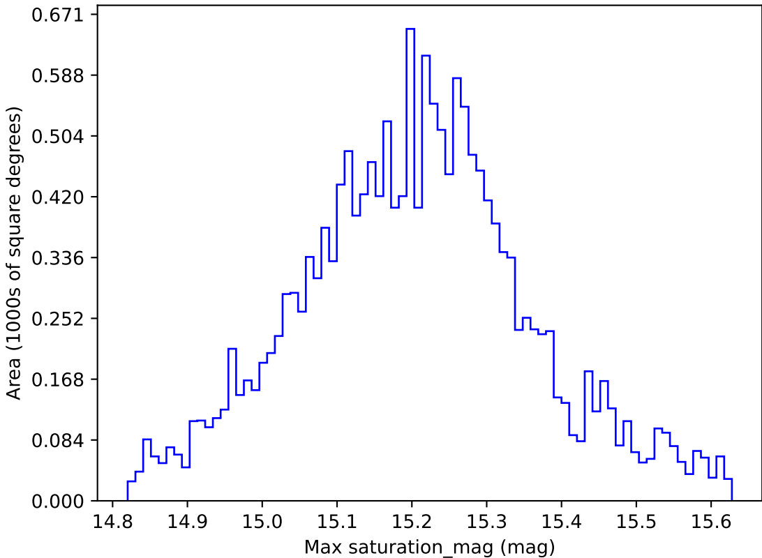
roll_pause_mjdp60_v3.4_10yrs WFD z band: Max saturation_mag
