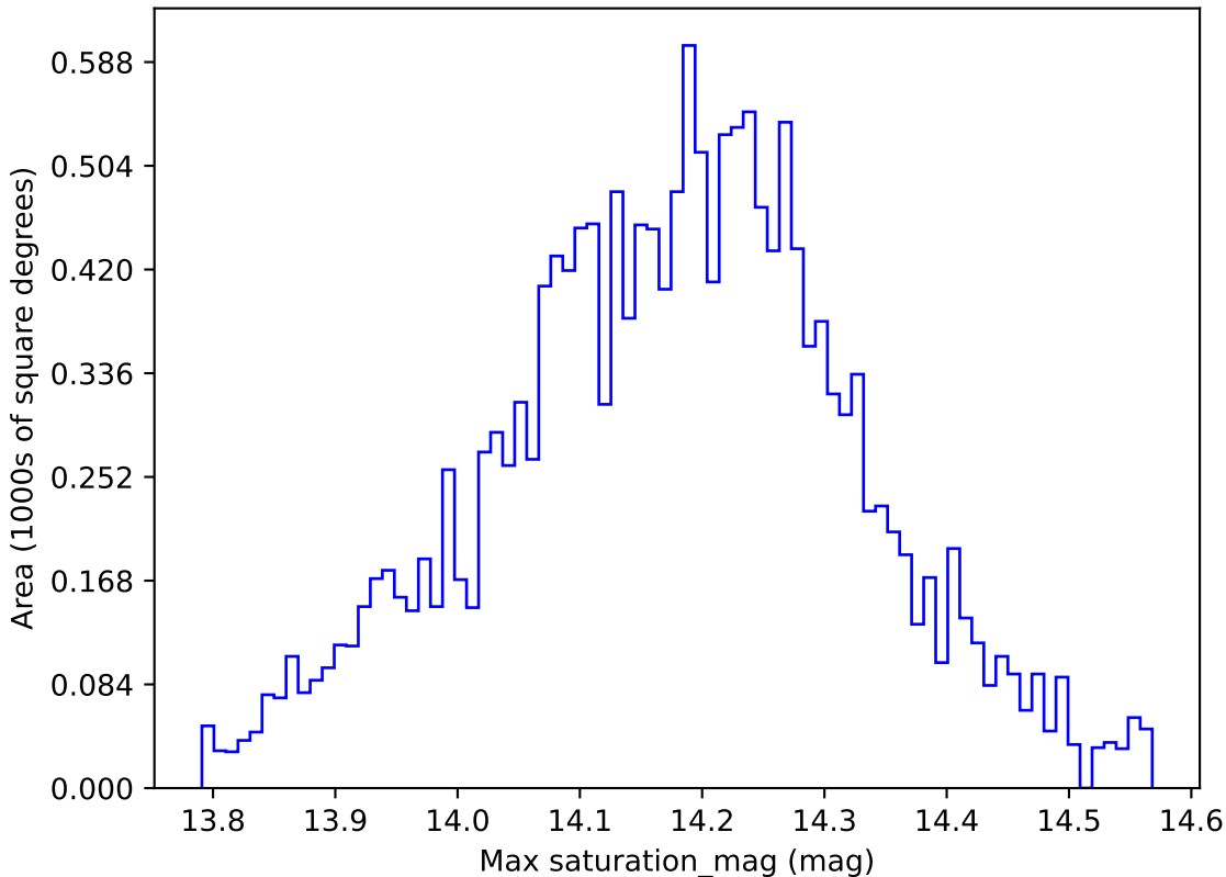
roll_pause_mjdp60_v3.4_10yrs WFD y band: Max saturation_mag
