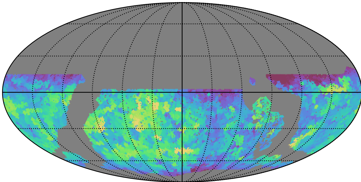
roll_pause_mjdp60_v3.4_10yrs WFD r band: Max saturation_mag
