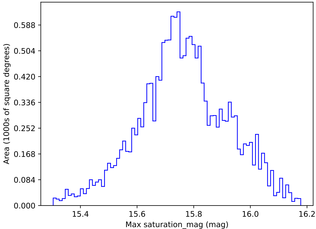
roll_pause_mjdp60_v3.4_10yrs WFD r band: Max saturation_mag
