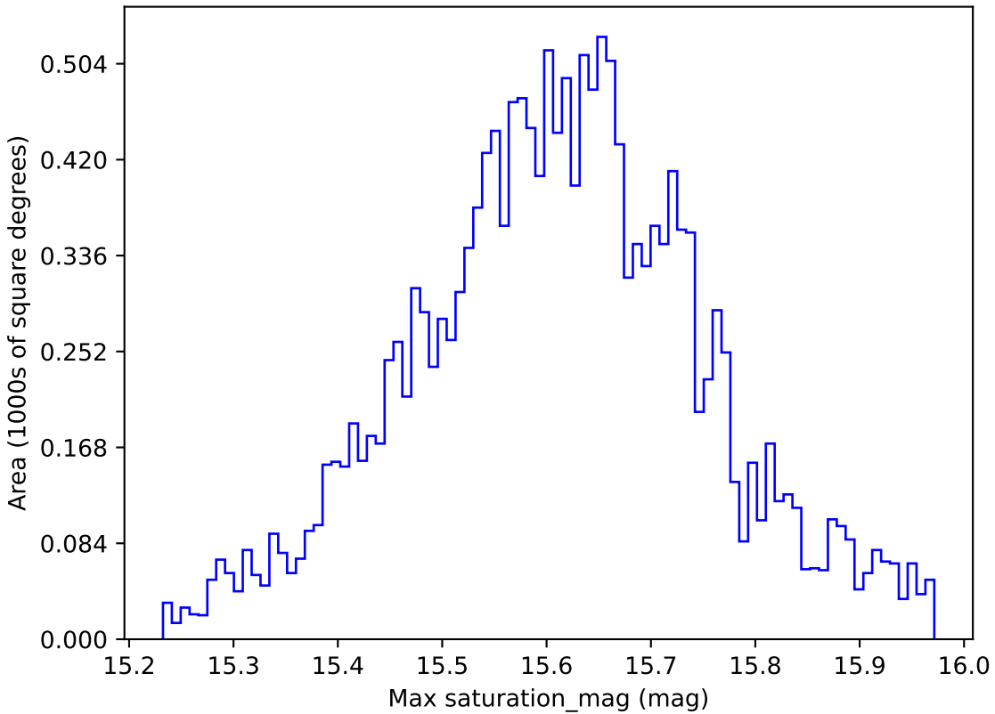
roll_pause_mjdp60_v3.4_10yrs WFD i band: Max saturation_mag
