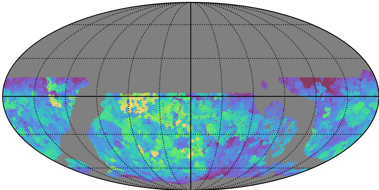
roll_pause_mjdp60_v3.4_10yrs WFD g band: Max saturation_mag
