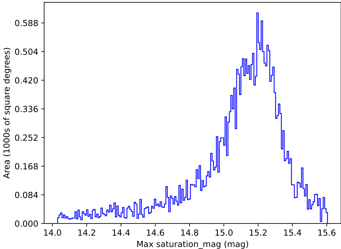
roll_pause_mjdp60_v3.4_10yrs All sky z band: Max saturation_mag
