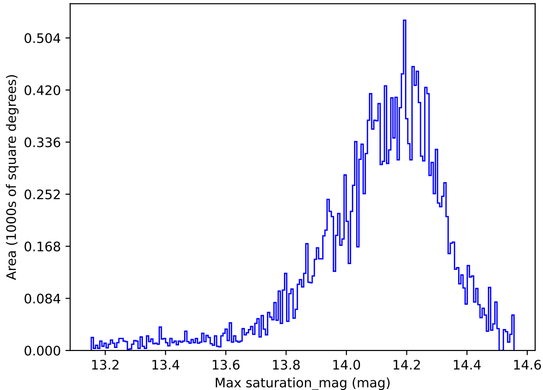
roll_pause_mjdp60_v3.4_10yrs All sky y band: Max saturation_mag
