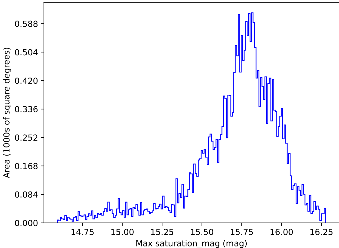
roll_pause_mjdp60_v3.4_10yrs All sky all bands: Max saturation_mag
