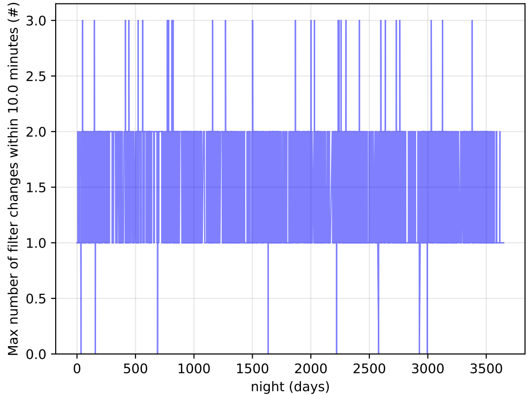
roll_pause_mjdp60_v3.4_10yrs Per Night: Max number of filter changes within 10.0 minutes
