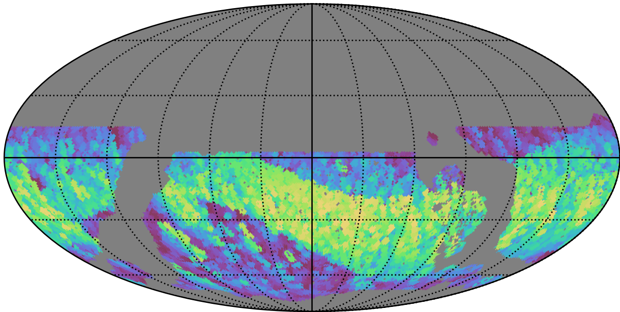
roll_pause_mjdp60_v3.4_10yrs WFD z band: Max normairmass
