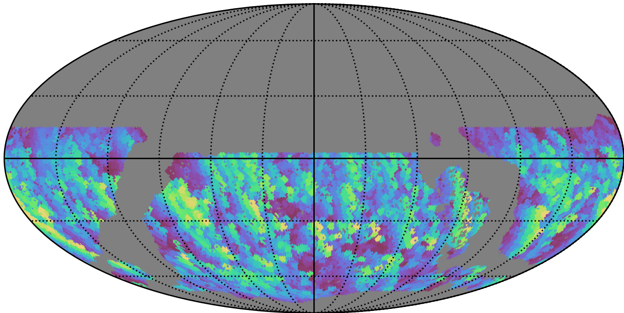
roll_pause_mjdp60_v3.4_10yrs WFD y band: Max normairmass
