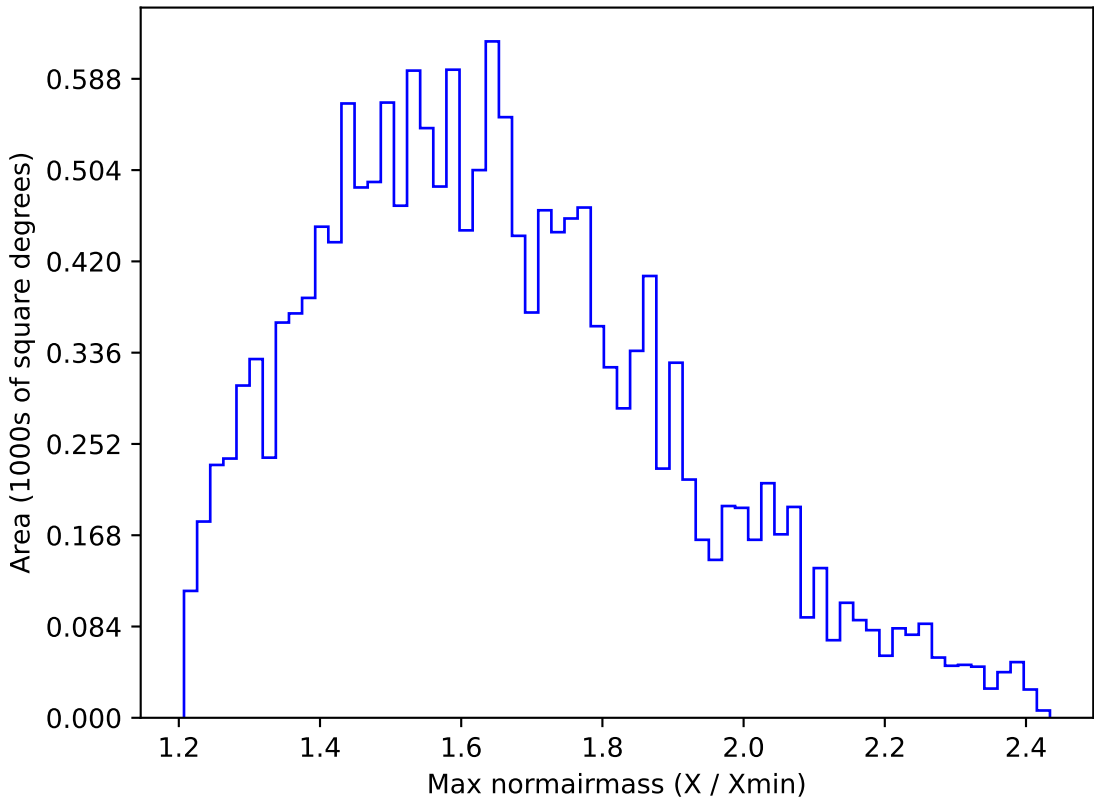
roll_pause_mjdp60_v3.4_10yrs WFD u band: Max normairmass
