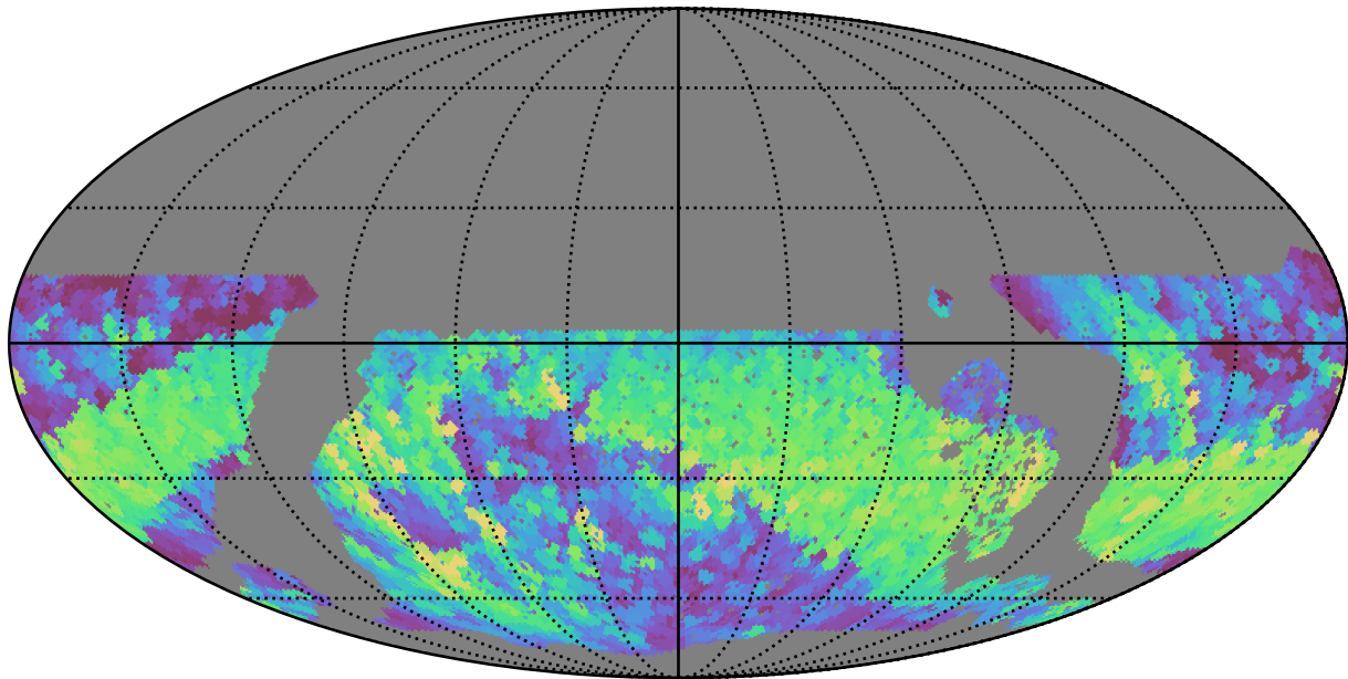
roll_pause_mjdp60_v3.4_10yrs WFD r band: Max normairmass
