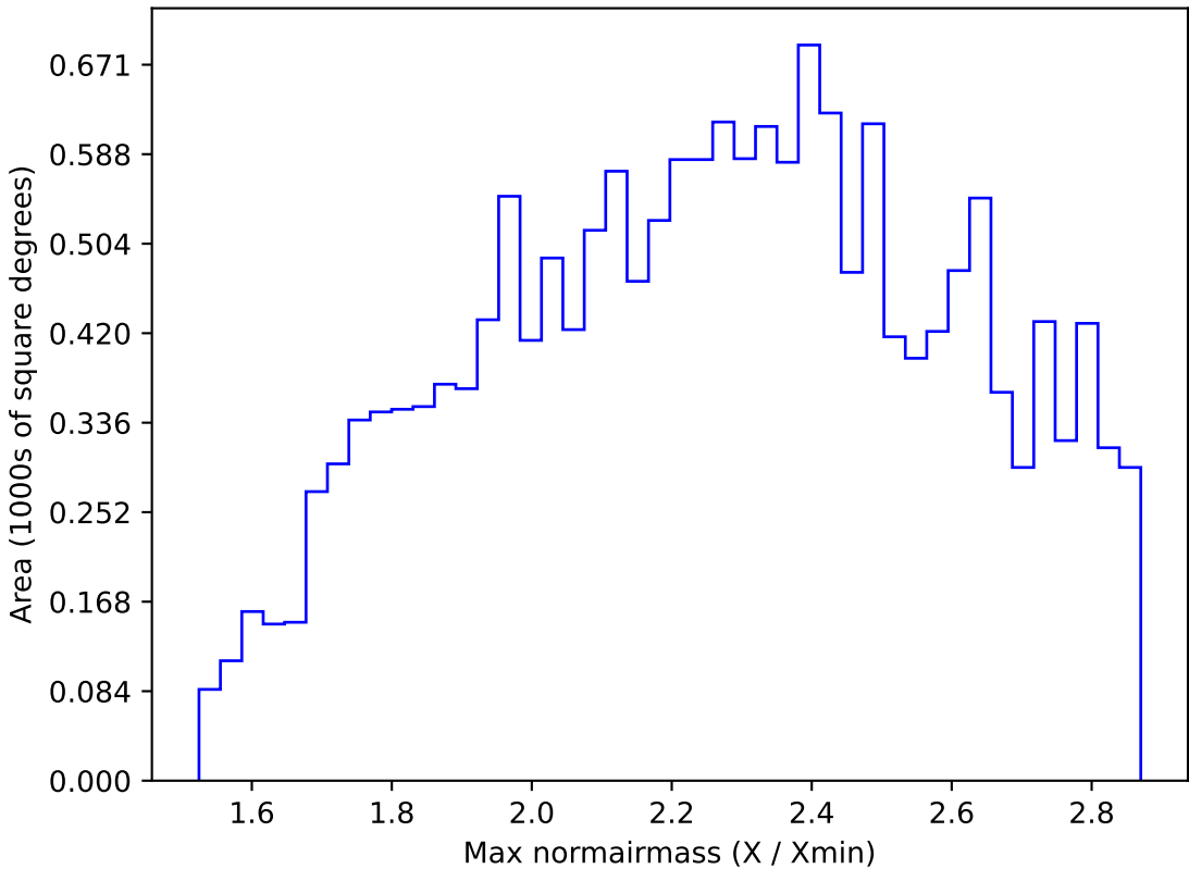
roll_pause_mjdp60_v3.4_10yrs WFD i band: Max normairmass
