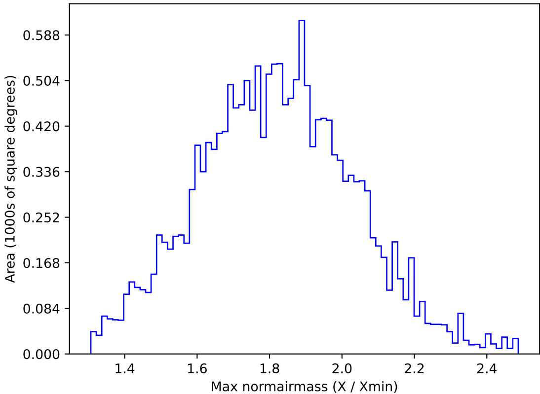
roll_pause_mjdp60_v3.4_10yrs WFD g band: Max normairmass
