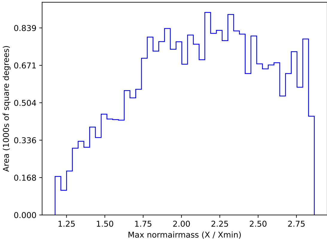
roll_pause_mjdp60_v3.4_10yrs All sky z band: Max normairmass
