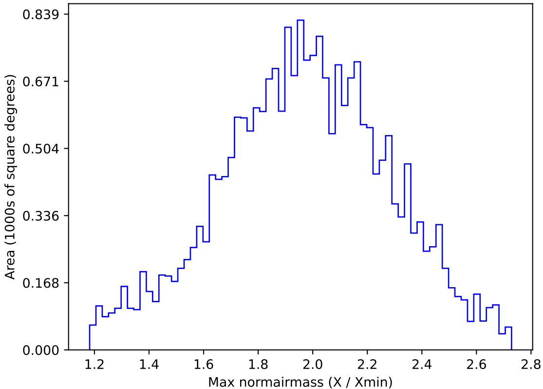
roll_pause_mjdp60_v3.4_10yrs All sky y band: Max normairmass
