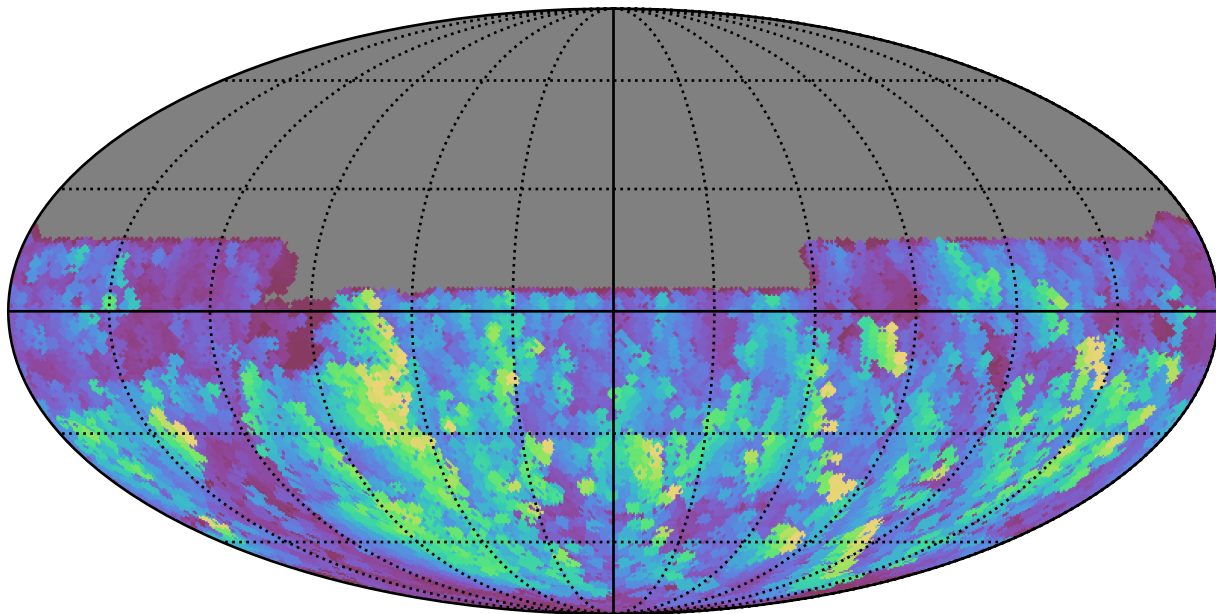
roll_pause_mjdp60_v3.4_10yrs All sky u band: Max normairmass
