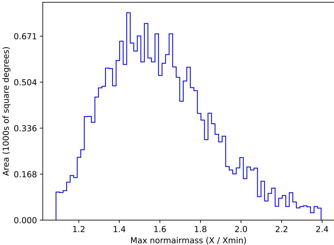
roll_pause_mjdp60_v3.4_10yrs All sky u band: Max normairmass
