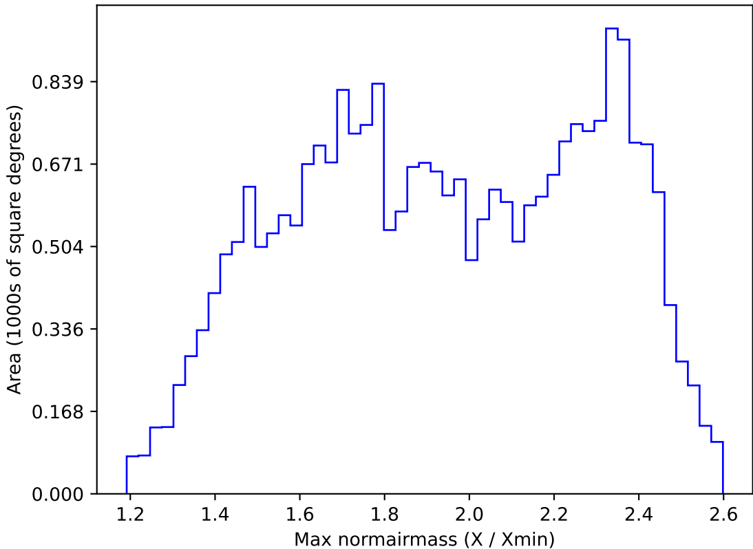
roll_pause_mjdp60_v3.4_10yrs All sky r band: Max normairmass
