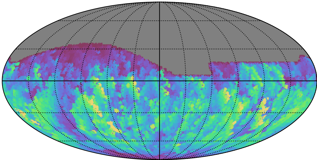
roll_pause_mjdp60_v3.4_10yrs All sky g band: Max normairmass
