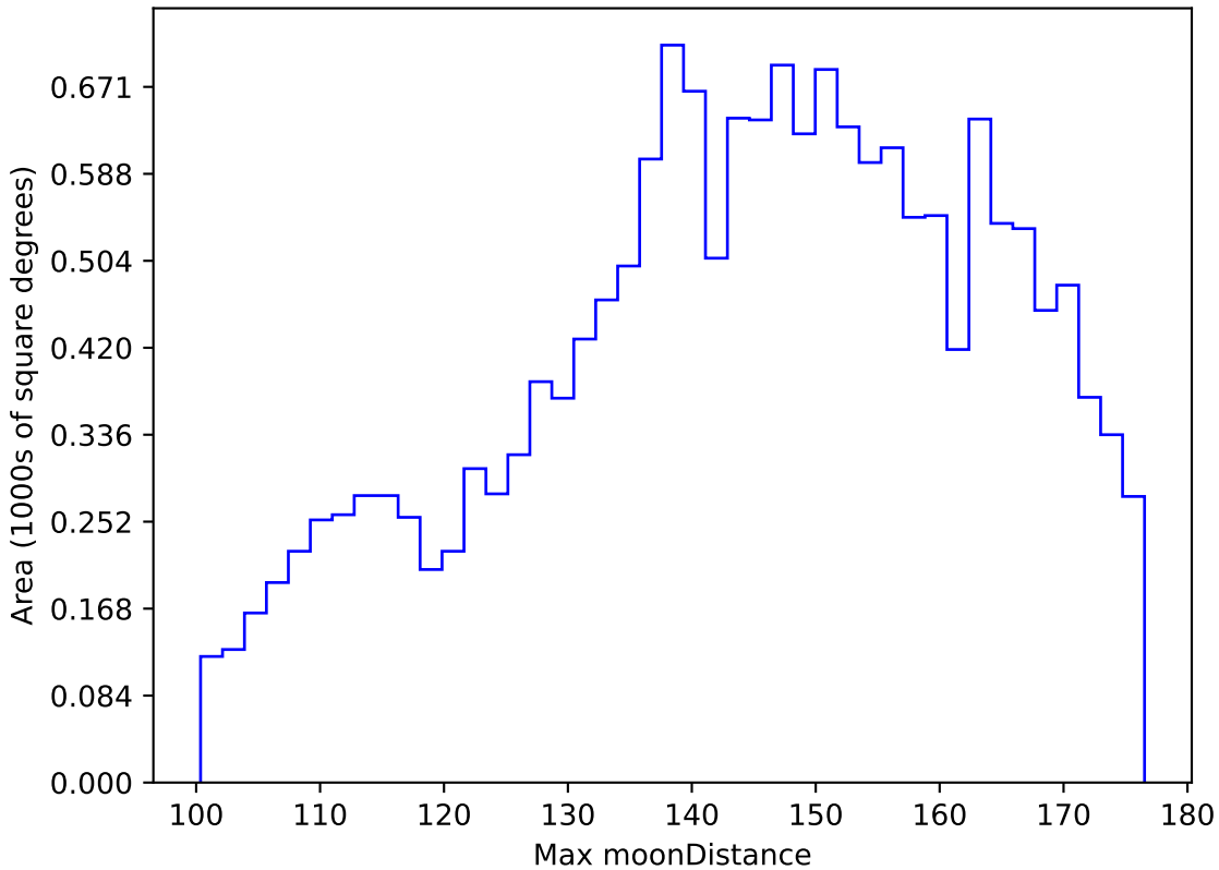
roll_pause_mjdp60_v3.4_10yrs WFD y band: Max moonDistance
