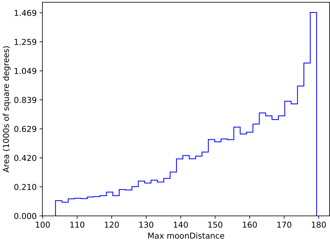
roll_pause_mjdp60_v3.4_10yrs WFD r band: Max moonDistance
