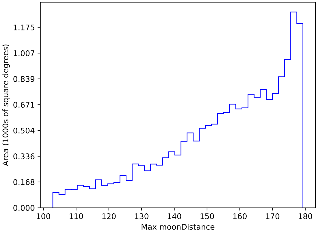
roll_pause_mjdp60_v3.4_10yrs WFD i band: Max moonDistance
