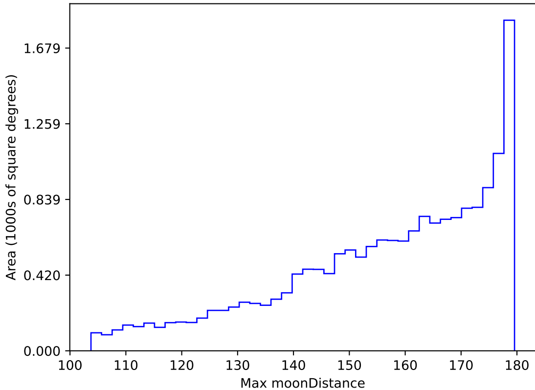
roll_pause_mjdp60_v3.4_10yrs WFD all bands: Max moonDistance
