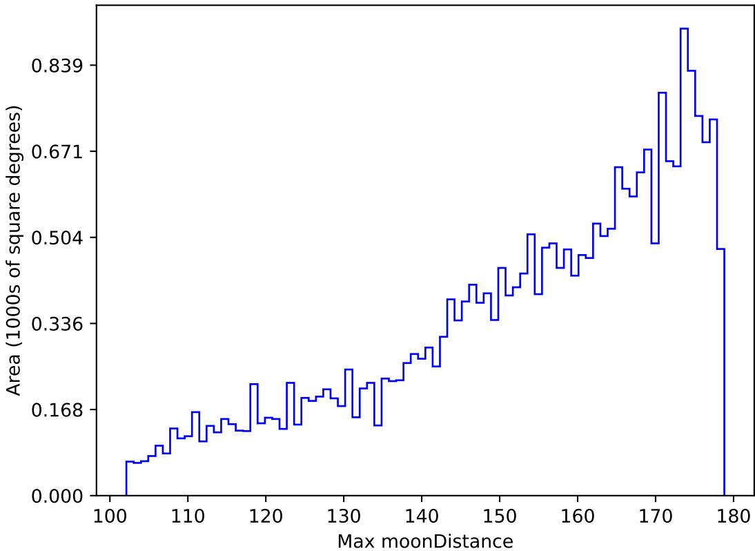
roll_pause_mjdp60_v3.4_10yrs All sky z band: Max moonDistance
