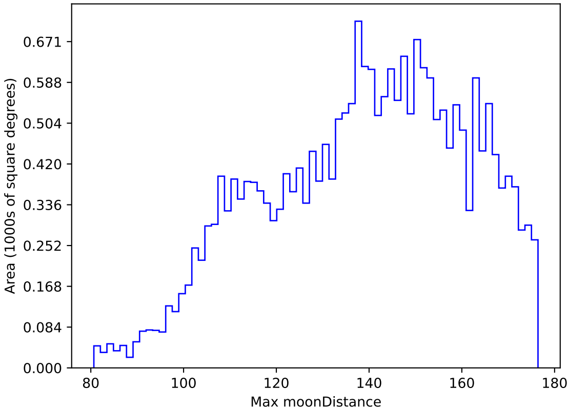
roll_pause_mjdp60_v3.4_10yrs All sky y band: Max moonDistance
