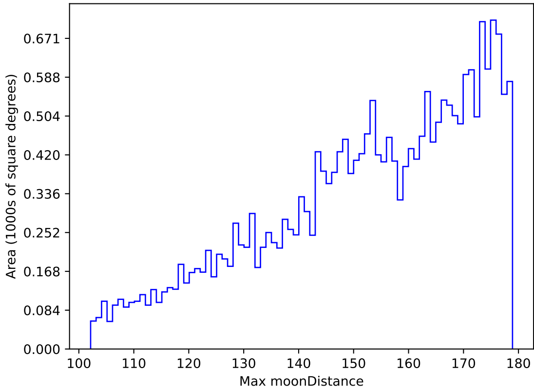
roll_pause_mjdp60_v3.4_10yrs All sky u band: Max moonDistance
