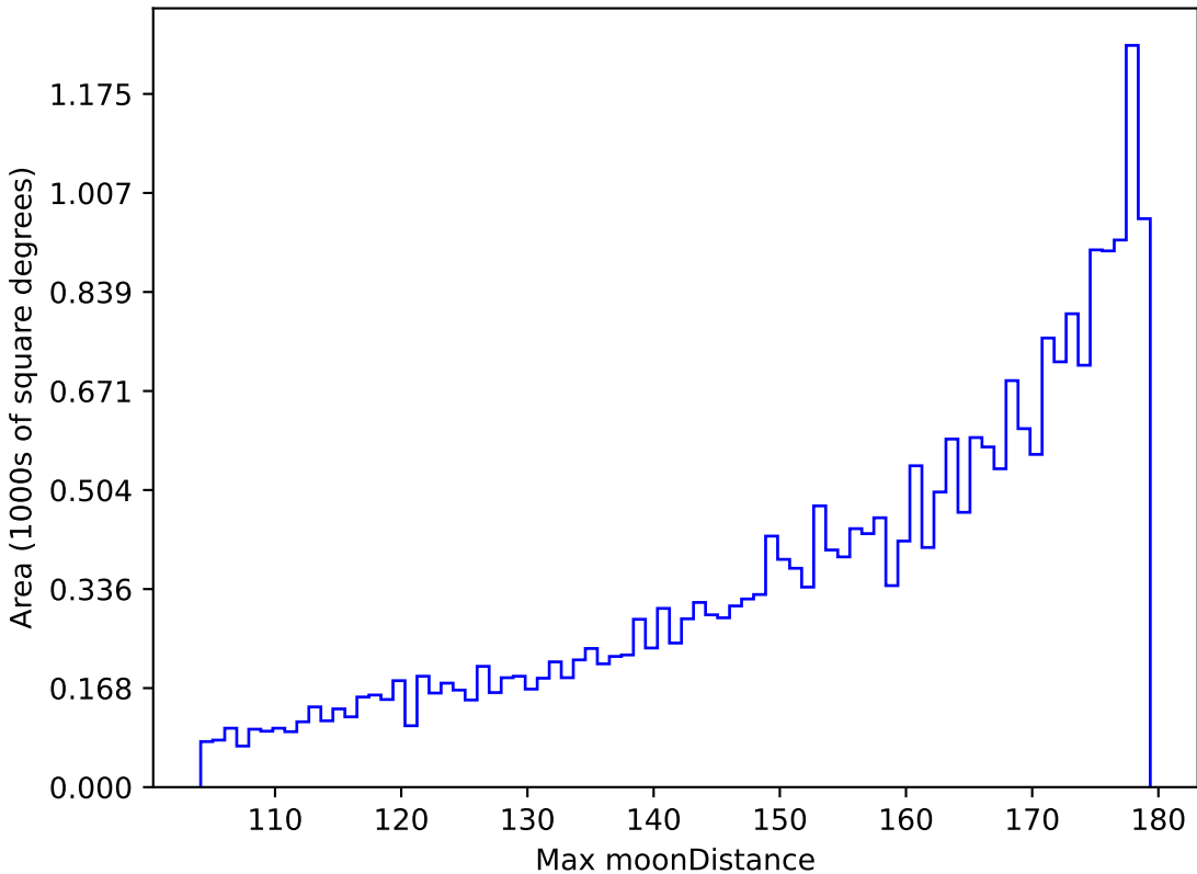
roll_pause_mjdp60_v3.4_10yrs All sky r band: Max moonDistance
