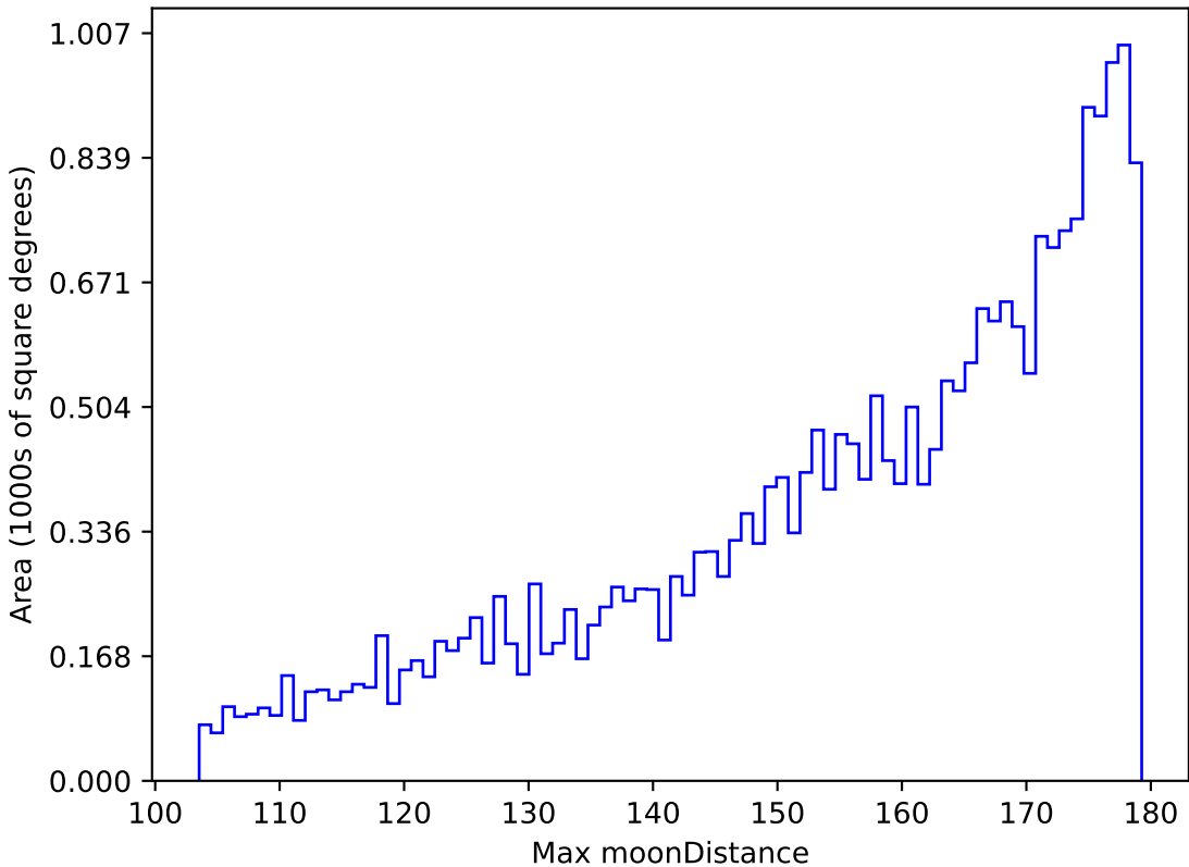
roll_pause_mjdp60_v3.4_10yrs All sky i band: Max moonDistance
