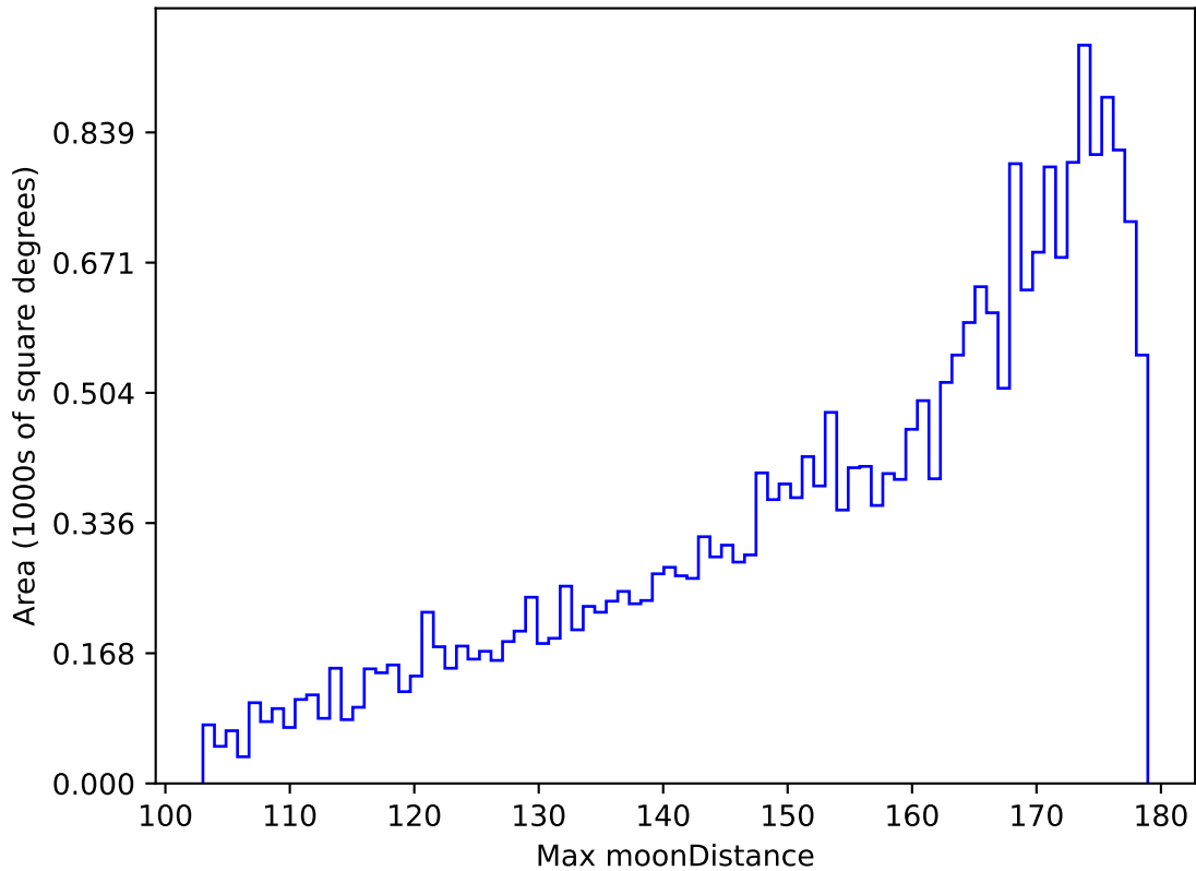
roll_pause_mjdp60_v3.4_10yrs All sky g band: Max moonDistance
