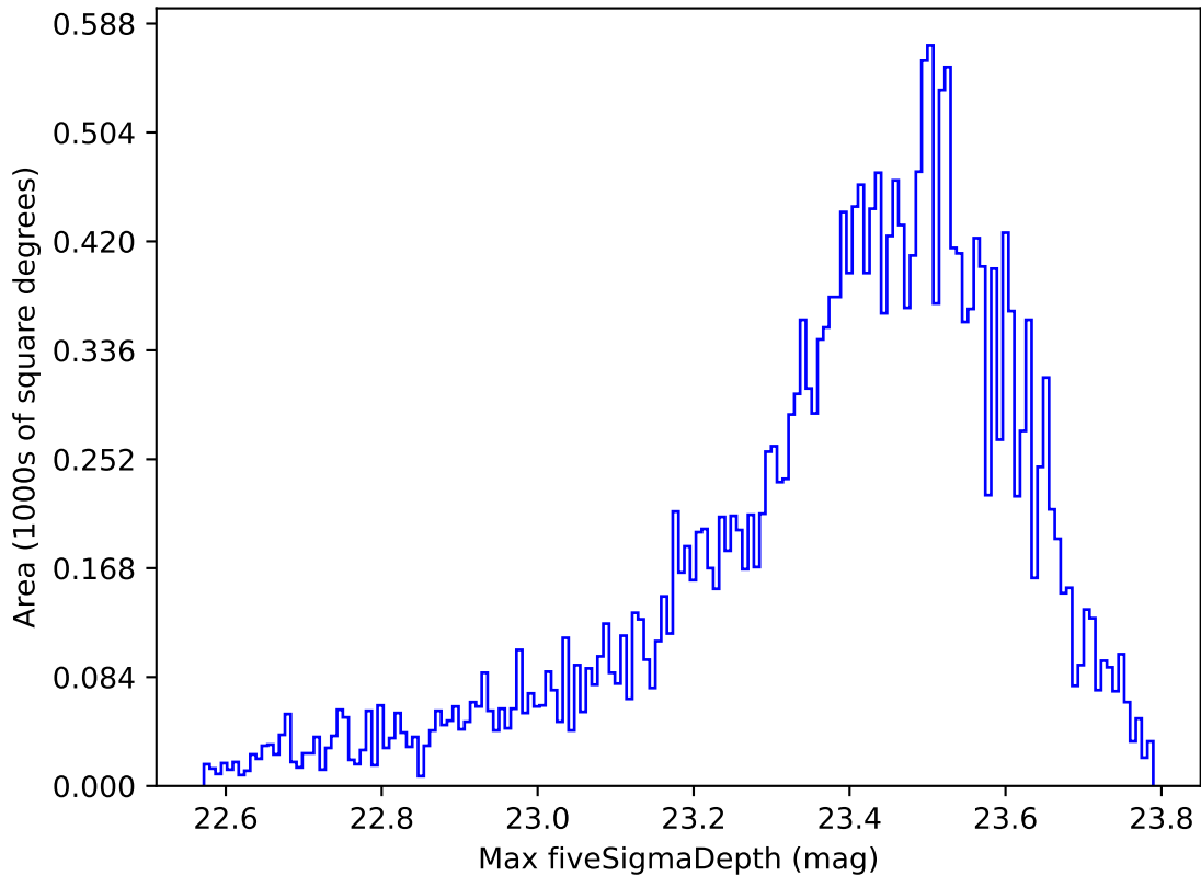
roll_pause_mjdp60_v3.4_10yrs Yr 1 z band: Max fiveSigmaDepth
