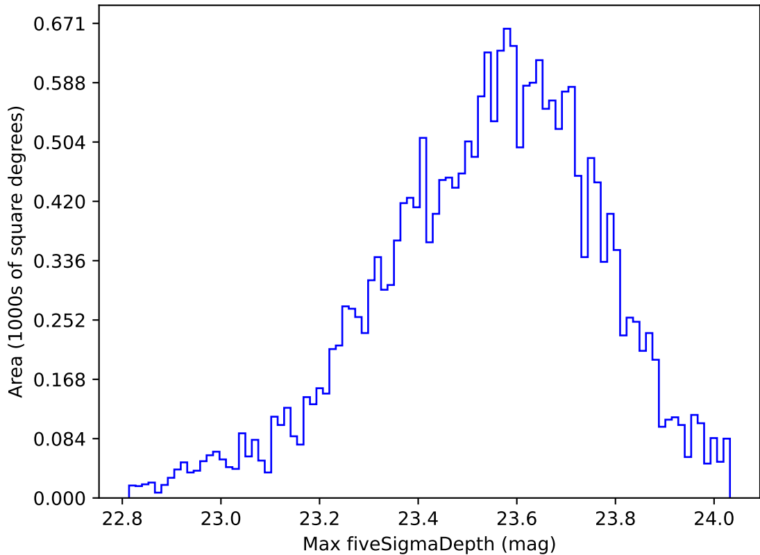
roll_pause_mjdp60_v3.4_10yrs Yr 1 u band: Max fiveSigmaDepth
