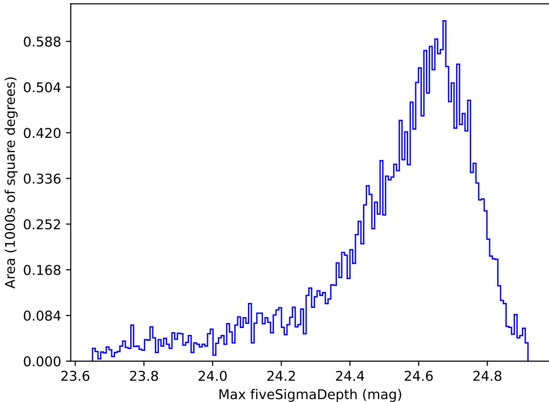
roll_pause_mjdp60_v3.4_10yrs Yr 1 r band: Max fiveSigmaDepth
